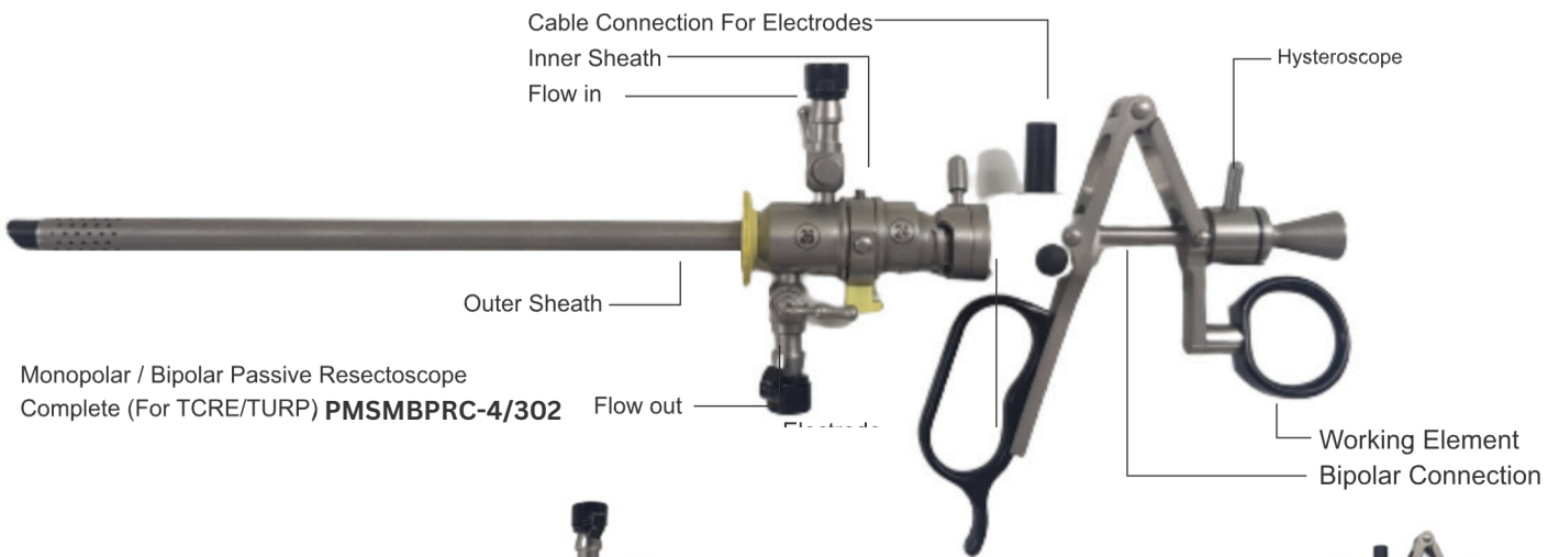
Working Element Active & Passive Resectoscope Monopolar / Bipolar
